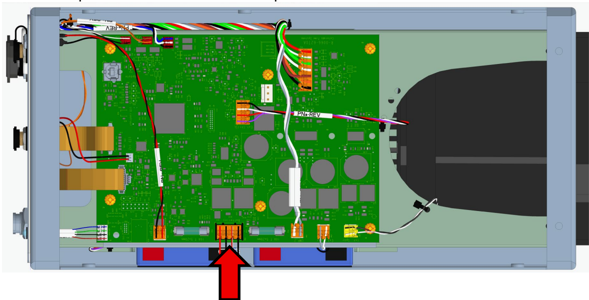
Battery Cable Connection
