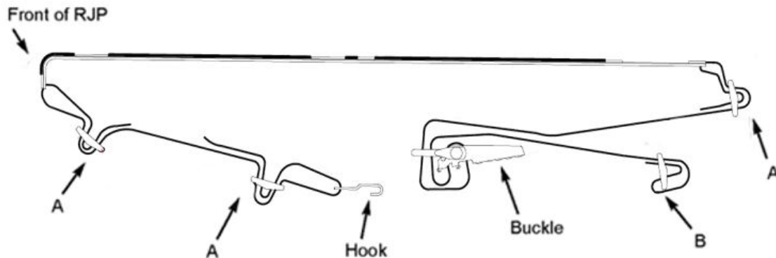
Figure 1 – Assembled Relay Judging Platform with mounting straps
