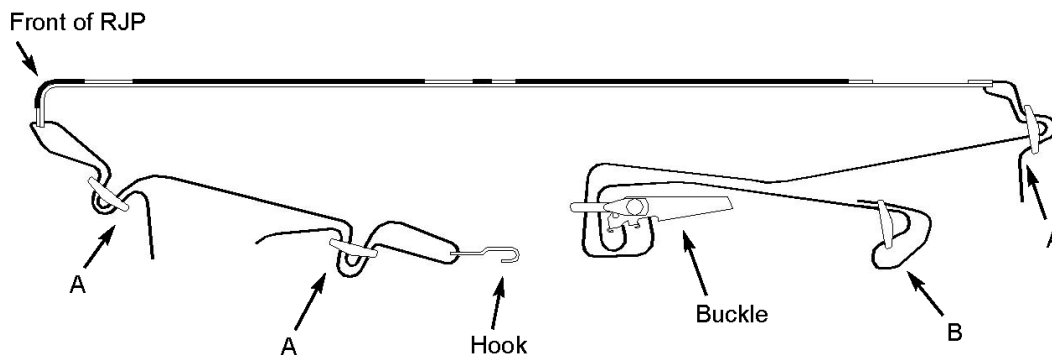
Figure 1 – Assembled Relay Judging Platform with mounting straps
